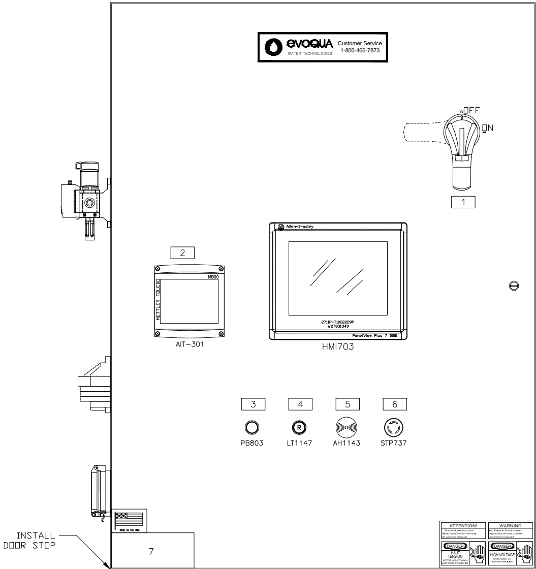
PANEL LAYOUT 48"x36"x12" [1219 X 914 X 305]
